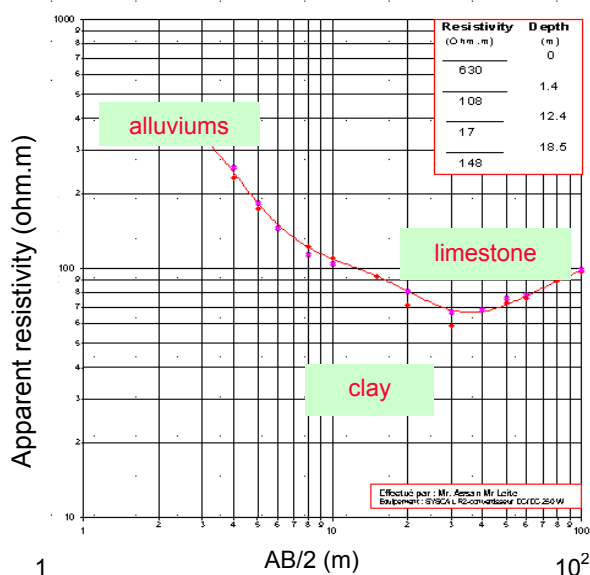
Fig 2: TWO LAYER MASTER CURVES FOR SCHLUMBERGER 1D SOUNDINGS
